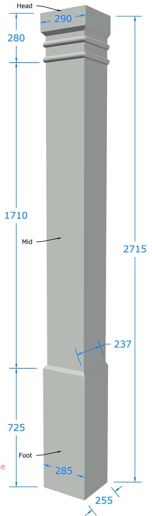
Maximum Sizes
